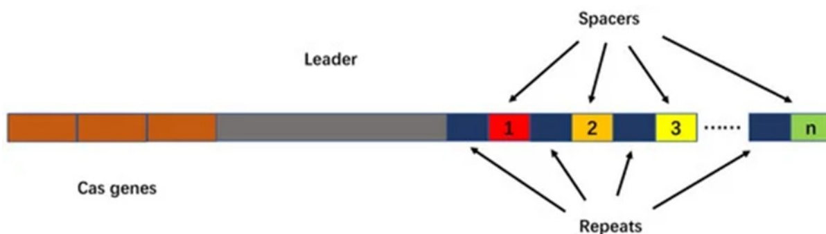
Figure 2. CRISPR-Cas locus structure diagram. CRISPR-Cas includes transactivating crRNA, genes encoding Cas-related proteins (Cas genes), repeat sequences and spacer sequences.
