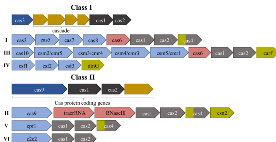
Figure 1. Functional organization of CRISPR systems.
